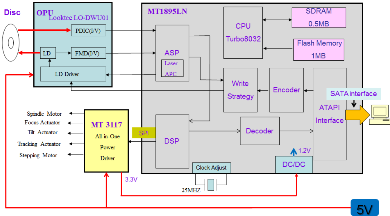
DS-8ABSH Block Diagram
